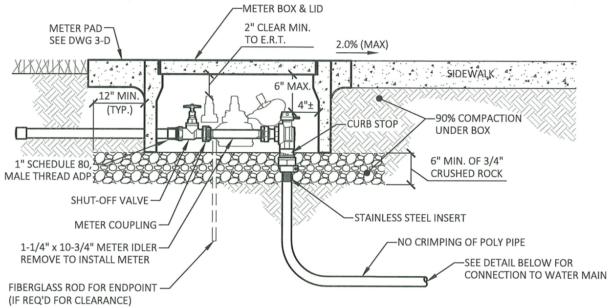
SECTION (SHOW W/IDLER)
